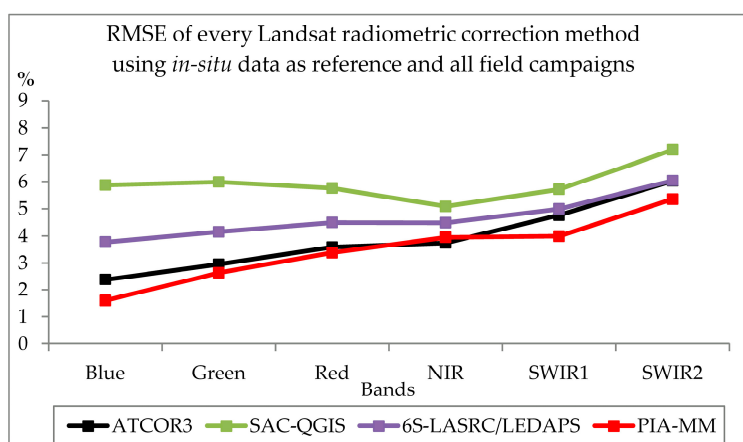
Figure 9. Band-by-band Root Mean Square Error of each radiometric correction method analyzed for Landsat images, grouping all dates.
